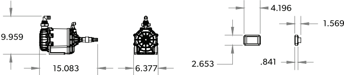
BOOSTER PUMP
