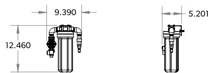
PRE FILTERS
