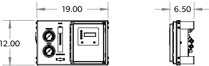
CONTROL PANEL
