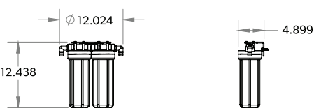
PRE FILTERS
