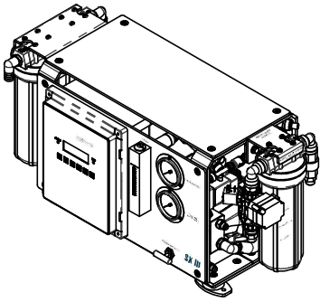
SXIII 6001 MEMBRANE VESSELS 600 GPD (2271LPD) / 25 GPH (95LPH)
