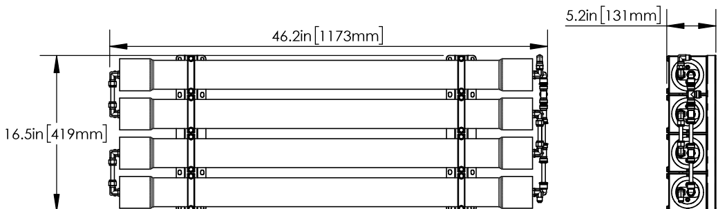
SXIII 2200 MEMBRANE VESSELS 2200 GPD (8328LPD) 92GPH (347LPH)
